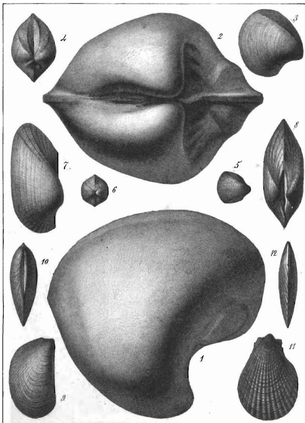
1, 2, Cyprina curvirostris , H. Coquand 7, 8, Arca Cymodoce , H. Coquand 3, 4, — modesta — 9, 10, Lima Eucharis — 5, 6, Cardium bidorsatum — 11, 12, Pecten Morellensis —
